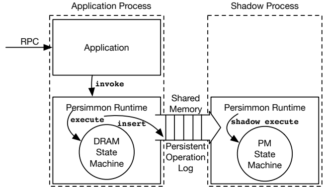
Figure 2: Persimmon runtime.
