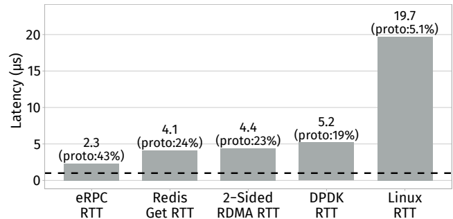
Figure 1: Reported RTTs of recent microsecond-scale systems, annotated with the percentage overhead that Protobuf serialization and deserialization of a single 1024 byte string (1.0 µs) would add (shown in the dashed line). Redis RTT comes from Arrakis [27], eRPC from eRPC [17], while the RDMA, DDPK and Linux RTTs are measured on the Demikernel. [42].
